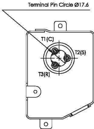
Junction Box Layout
