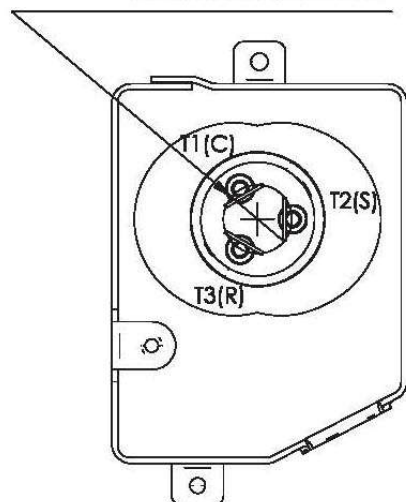
Junction Box Layout
