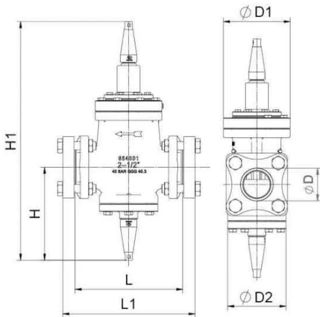
入口压力调节阀 Inlet Pressure Regulating Valve IPRV
